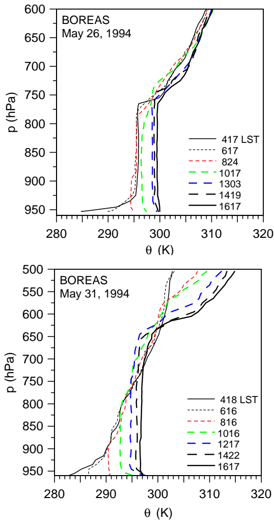
Figure 3. Profiles of potential temperature in the lower troposphere on May 26 and 31.
