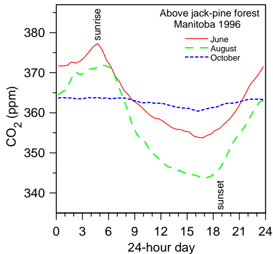
Figure 4. Monthly mean diurnal cycle of \text{CO}_2 for June, August and October for a boreal jack-pine site.
