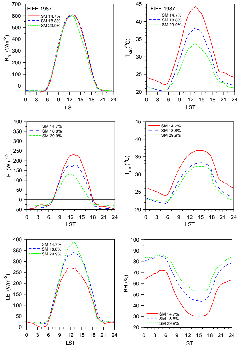
Figure 1. Diurnal cycle of net radiation ( R_n ), sensible heat flux ( H ) and latent heat flux ( LE ) (left panels); surface temperature, air temperature and relative humidity (right panels), stratified by percent volumetric soil moisture in first 10cm of the soil.
