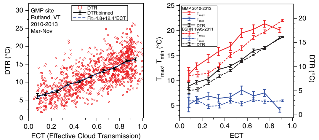
Figure 9. Relation between ECT and DTR (left: daily data) and (right) comparison between T_{max} , T_{min} and DTR at GMP site with BSRN site near Regina, Saskatchewan.
