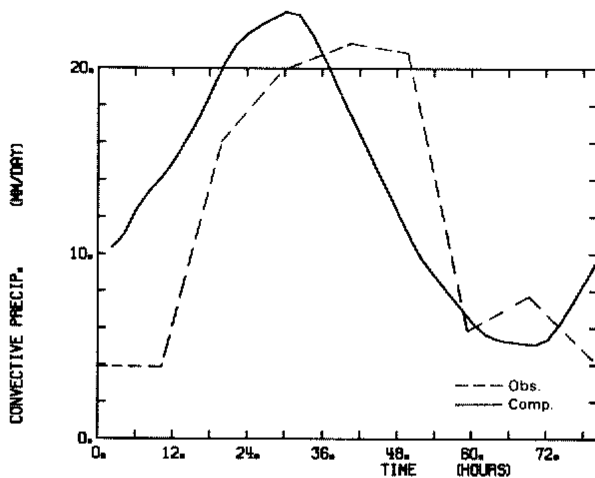
Figure 7. Comparison of observed and computed rainfall.
