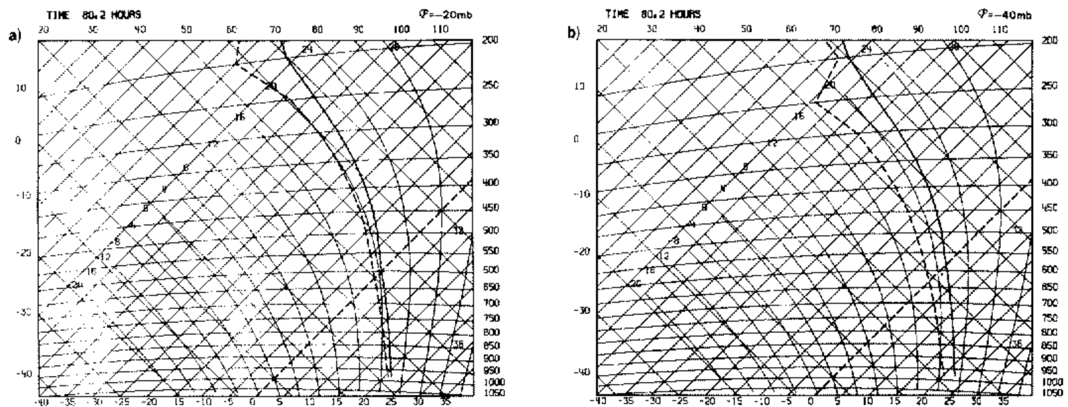
Figure 11. Model thermodynamic structure at 80h for the subsaturation parameter: (a) \mathcal{P} = -20\text{mb} ; (b) \mathcal{P} = -40\text{mb} ( \alpha = 1 , \tau = 2\text{h} ).
