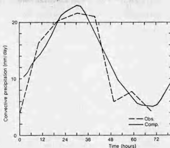
Figure 7. Comparison of observed and computed rainfall.
