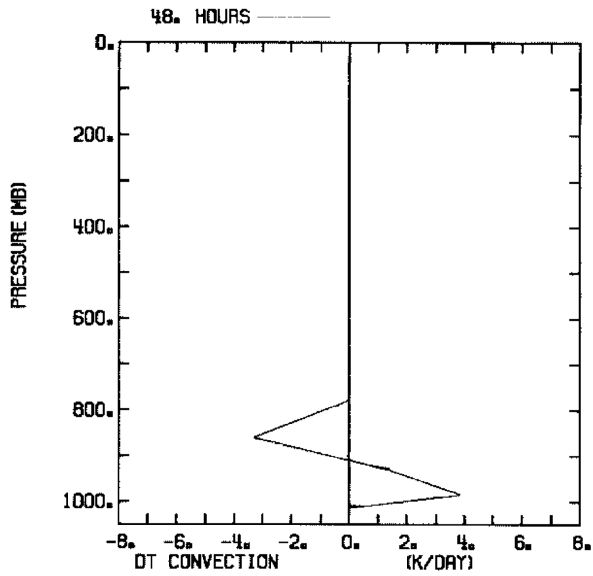
Figure 19. Computed ATEX convective heat source.
