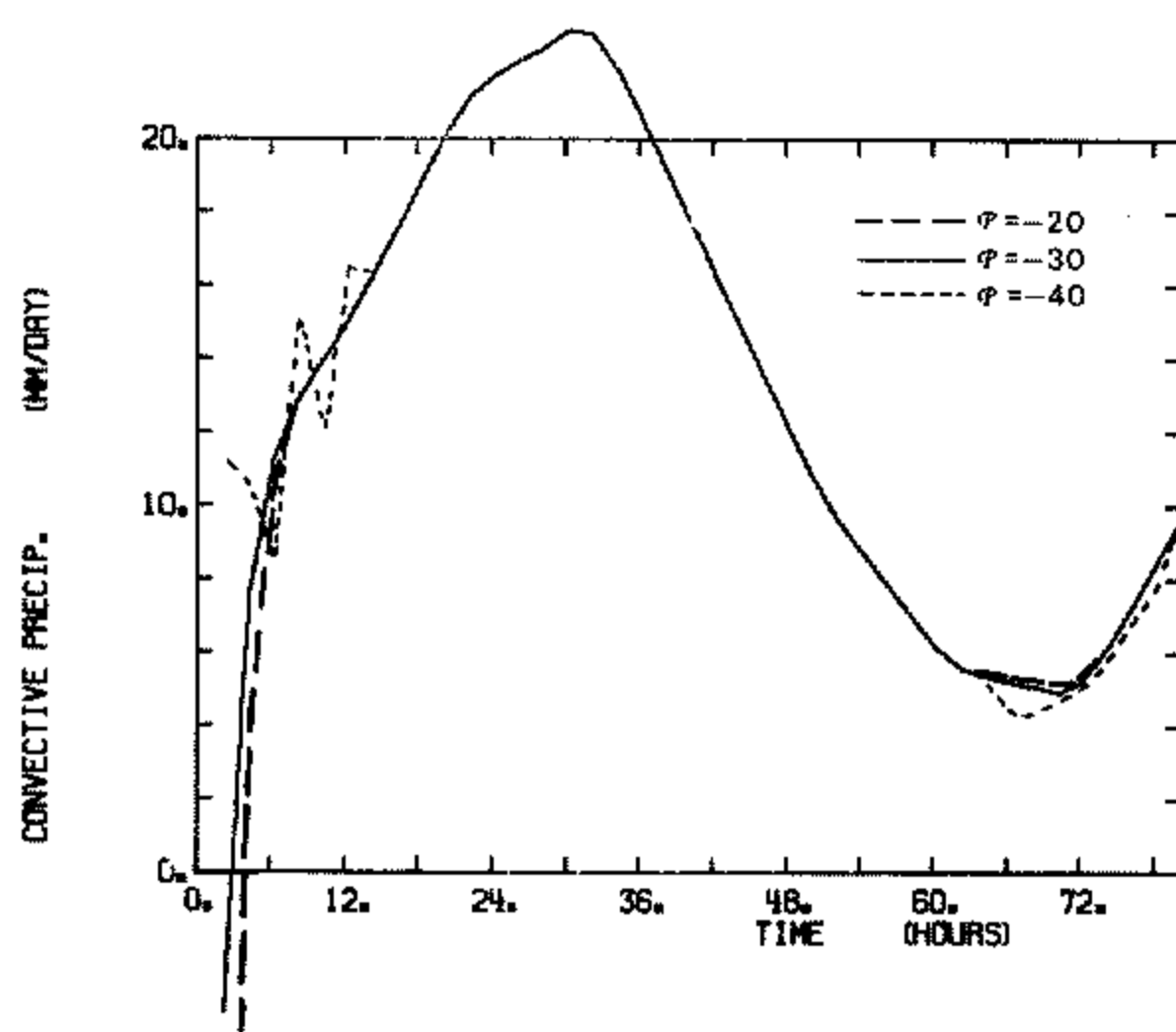
Figure 12. Model precipitation for \mathcal{P} = -20, -30 and -40 mb (with \alpha = 1.0 and \tau = 2 hours).
