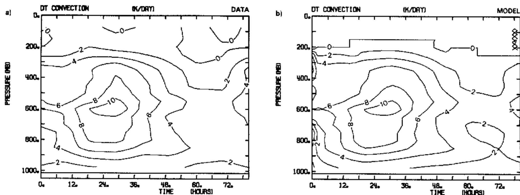
Figure 5. Comparison of (a), diagnosed and (b), computed convective heating for GATE wave data.
