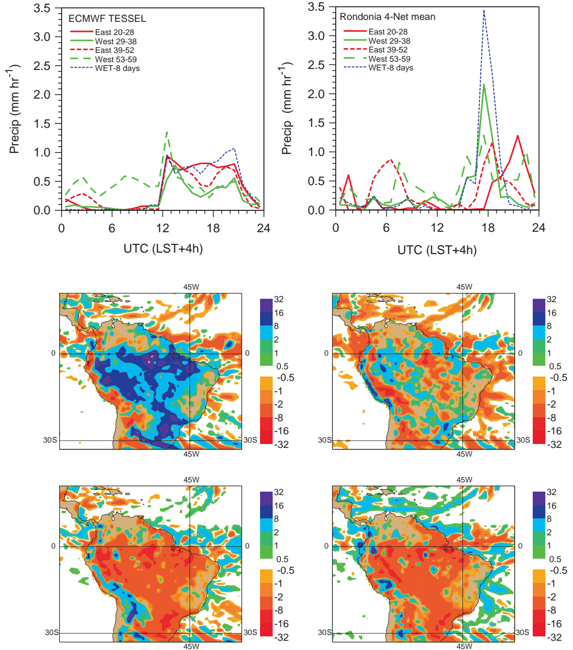
Figure 1. (top left) Mean diurnal cycle of precipitation over Rondônia for five convective classifications for current ECMWF model; (top right) observed mean diurnal cycle of precipitation over Rondônia, an average of four rain gage networks. (lower panels) Diurnal cycle of precipitation anomaly from daily total over South America from operational ECMWF model for 1–7 February 1999. Shown are the 6-hour averages from 1200–1800 UTC (8–14 LST (center left), 1800–0000 UTC (center right), 0000–0600 UTC (bottom left), 0600–1200 UTC (bottom right). The units are mm d -1 .
