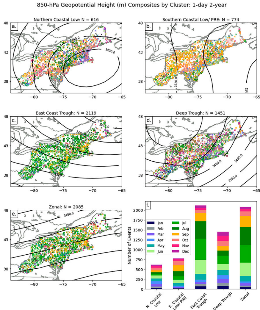
FIG. A1. As in Fig. 5, but for a smaller geographical domain ( 36^{\circ} – 48^{\circ} N, 85^{\circ} – 65^{\circ} W).
