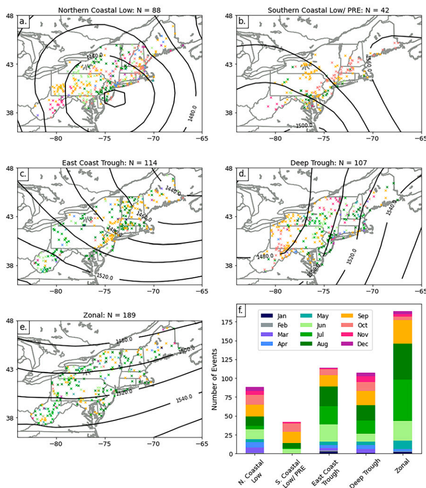
FIG. A2. As in Fig. 6, but for a smaller geographical domain ( 36^{\circ} – 48^{\circ} N, 85^{\circ} – 65^{\circ} W).
