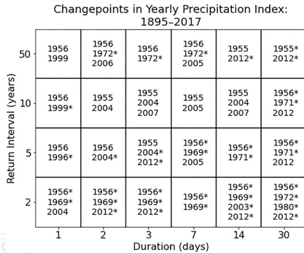
FIG. 3. Changepts identified in the yearly precipitation index time series from 1895 to 2017 for each duration–return interval combination. Years with an asterisk indicate that the changept was statistically significant to 95% confidence using Welch's unequal variances t test ( p < 0.05 ).
